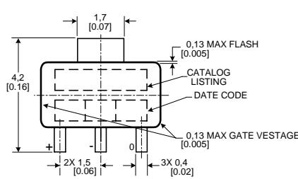
SS50AT SERIES MOUNTING DIMENSIONS (for reference only) mm/[in]
